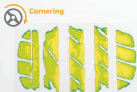
Traction force at cornering
